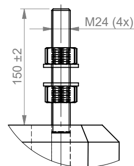
DETAIL D SCALE 1 : 5
