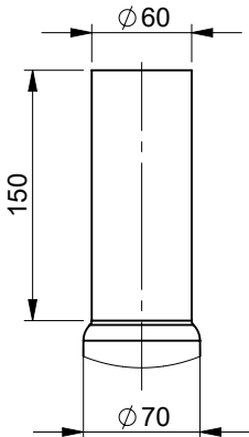
DETAIL E SCALE 1 : 5
