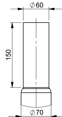
DETAIL E SCALE 1 : 5
