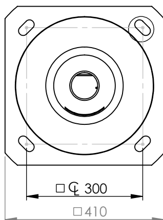
DETAIL C SCALE 1 : 2
