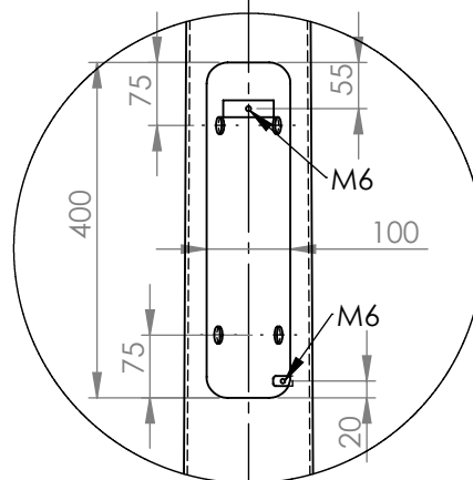
DETAIL B SCALE 1 : 10
