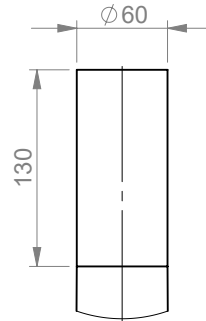
DETAIL A SCALE 1 : 5
