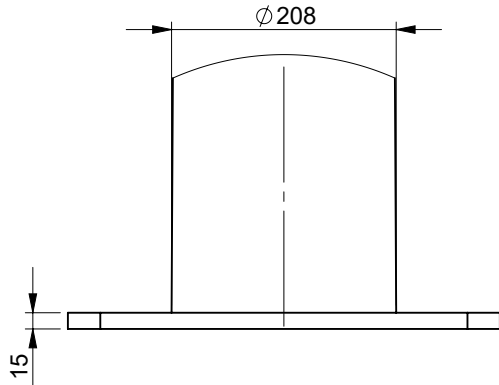
DETAIL B SCALE 1 : 7
